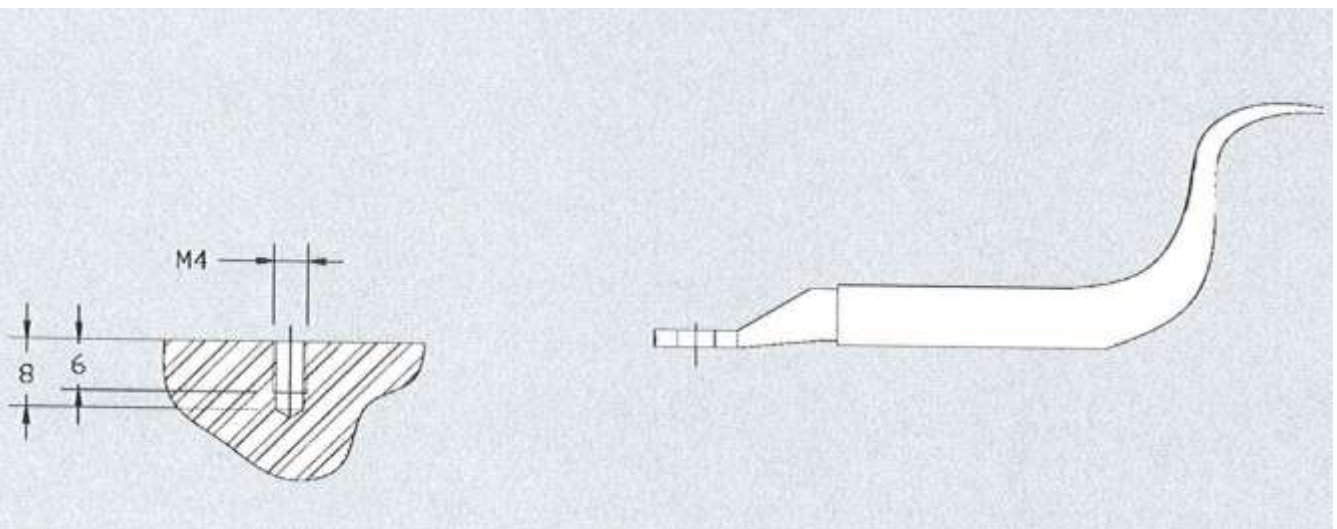
MFTC NOZ13, Fe-CuNi – ASA Standard Type J
