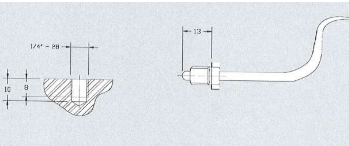
MFTC NOZ13, Fe-CuNi – ASA Standard Type J
